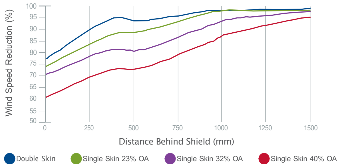
Average wind velocity reduction (%) with distance behind shield
