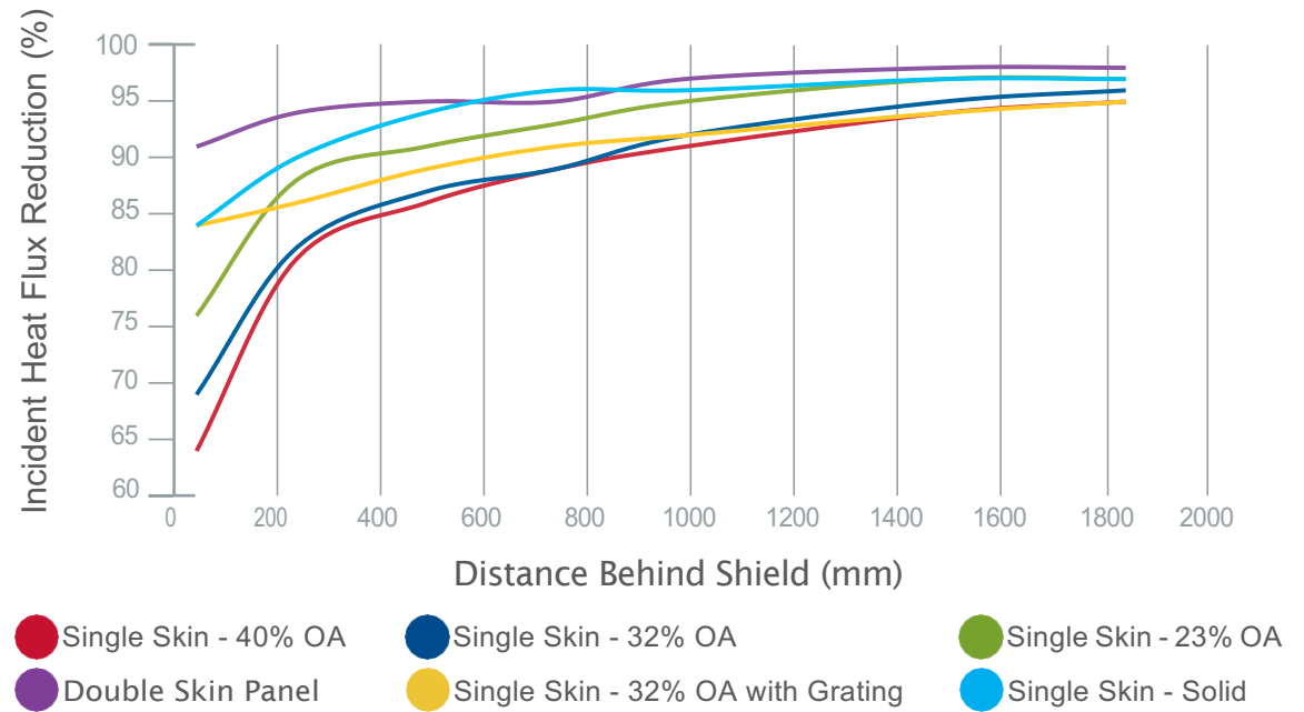
Incident heat flux reduction (%) with distance behind shield
